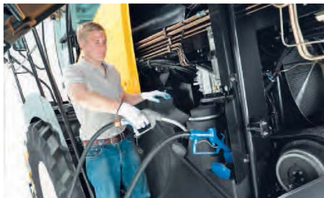
The fill openings for the fuel and 40 gallon AdBlue® tanks are conveniently located next to each other under the left side shield.
