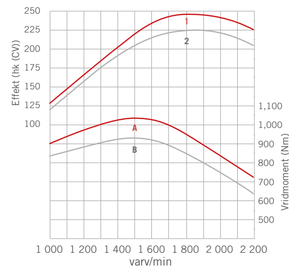
PUMA 200 CVX
